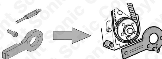
Component 1,3 & 6 - Crankshaft Alignment Tool
